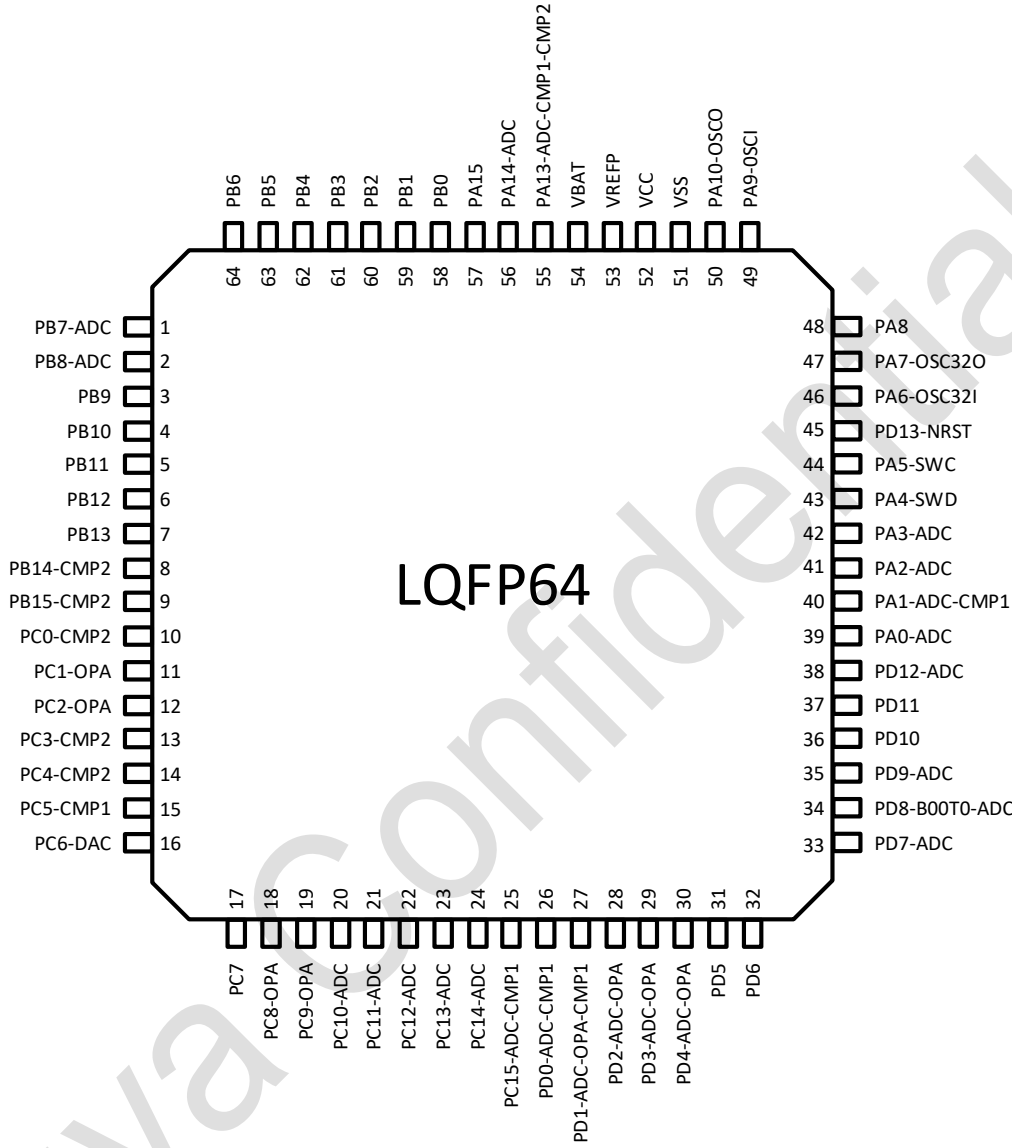
Figure 3-1 LQFP64 Pinout2 PY32L090R2xT7 (Top view)
