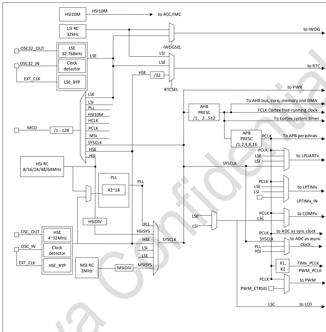
Figure 2-1 System clock structure diagram
