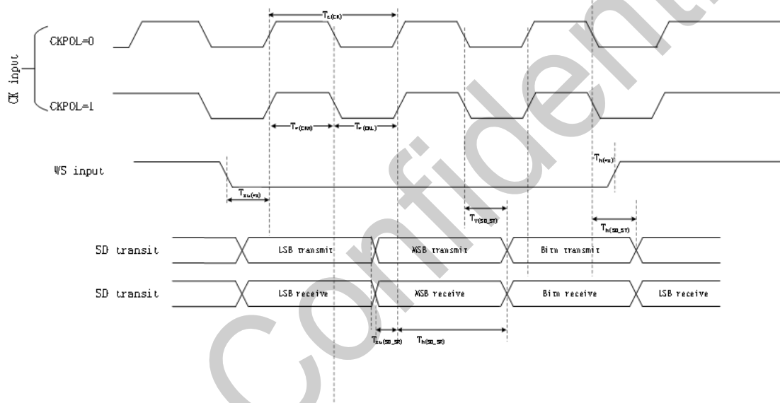
Figure 5-7 I²S timing diagram-Slave mode(Philips protocol )
