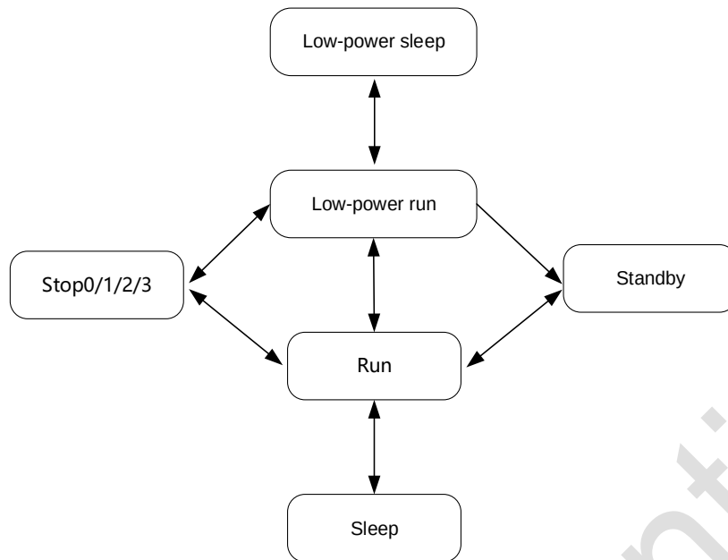
Figure 2-5 Power consumption state transition diagram
