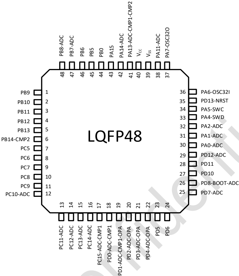
Figure 3-2 LQFP48 Pinout2 PY32L090C2xT7 (Top view)
